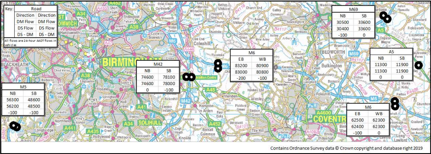
Figure 4.9: Forecast AADT Flows - M42 / M6 South East (2039)
