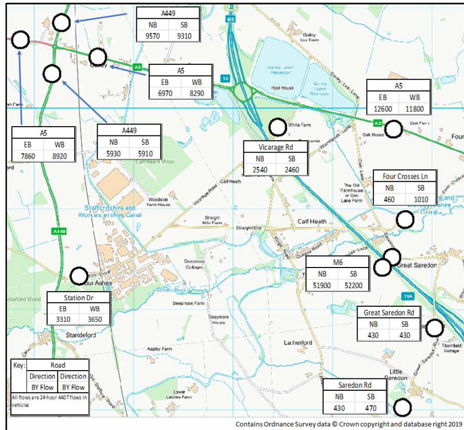
Figure 3.13: Baseline Model AADT Flows - A5 / M6 Junction 12 (2015)
