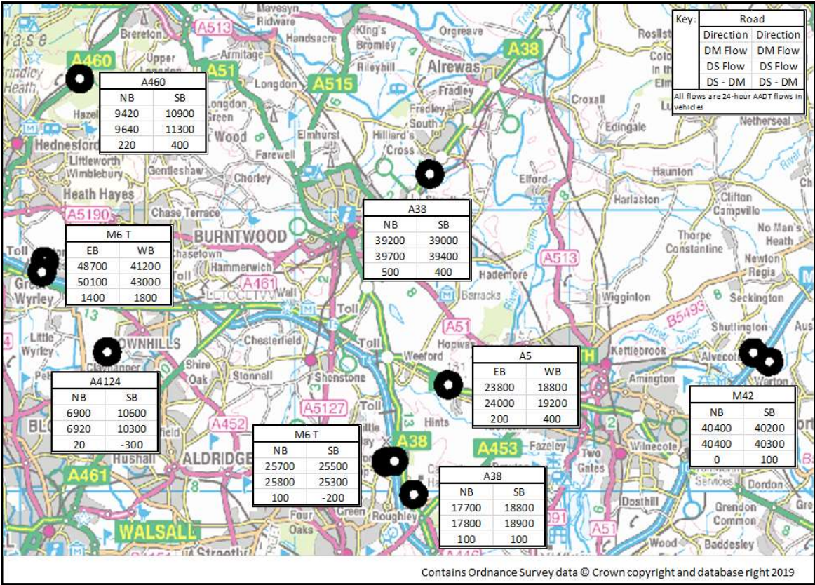
Figure 4.8: Forecast AADT Flows - M6 Toll / A5 East (2039)
