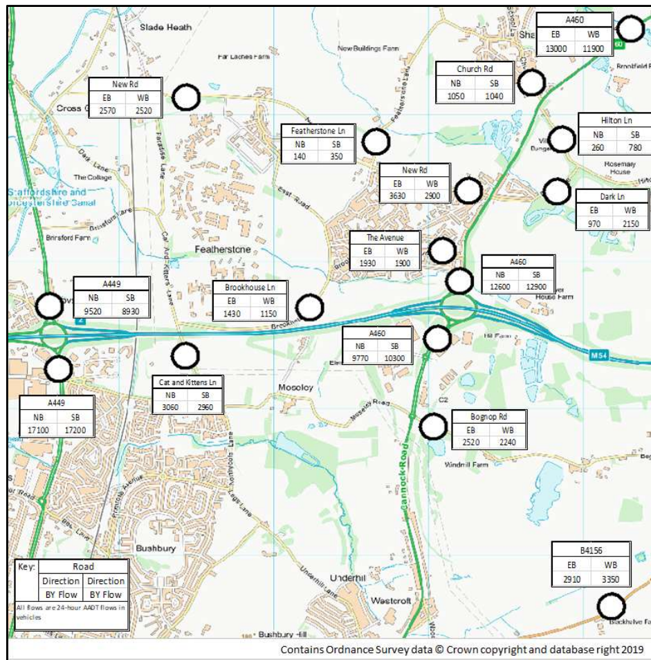
Figure 3.15: Baseline Model AADT Flows - M54 / A460 (2015)
