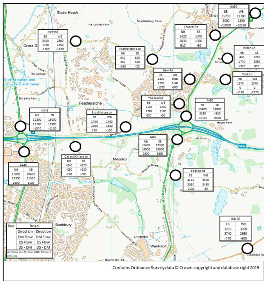
Figure 4.12: Forecast AADT Flows - M54 / A460 (2039)
