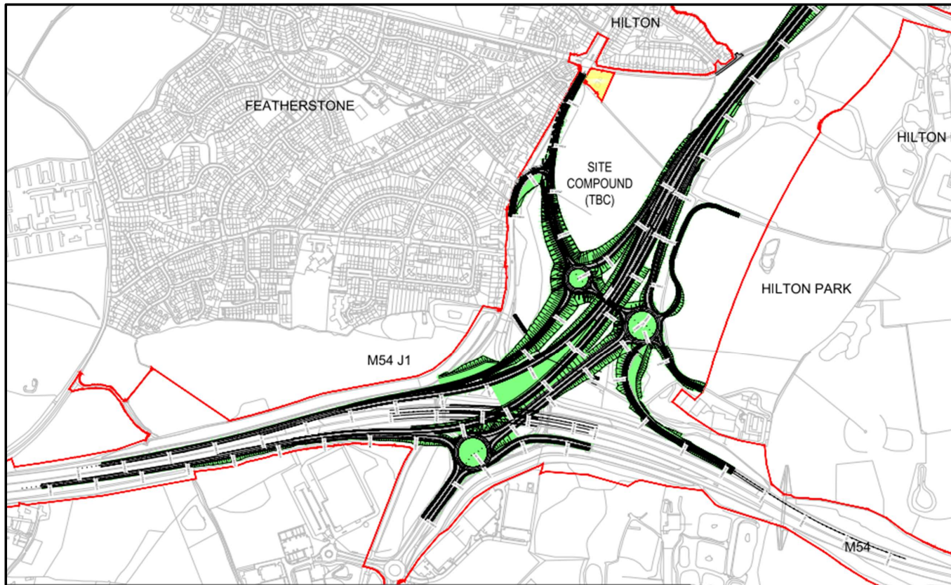
Figure 4.5: Improvements At M54 Junction 1
