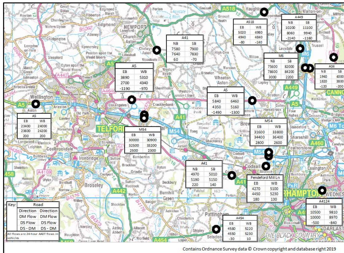
Figure 4.7: Forecast AADT Flows - M54 West (2039)
